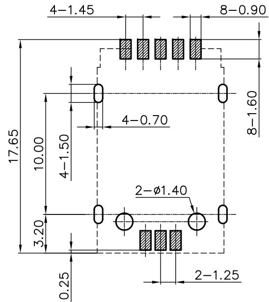
PCB Layout Diagram Top View
